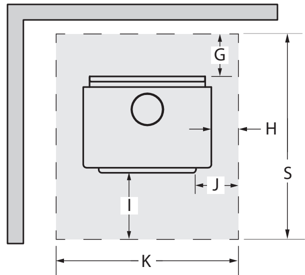
Figure 16: Protection de plancher
