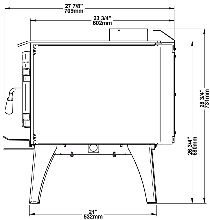
Figure 3: Side View
