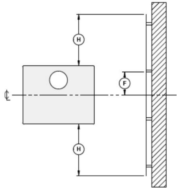
Figure 20: Heat shield clearances
