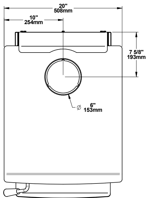
Figure 1: Top View
