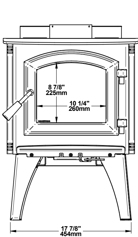
Figure 2: Front View
