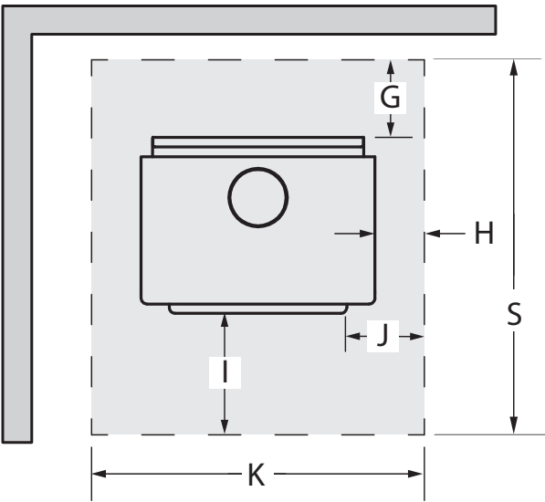
Figure 16: Floor Protection
