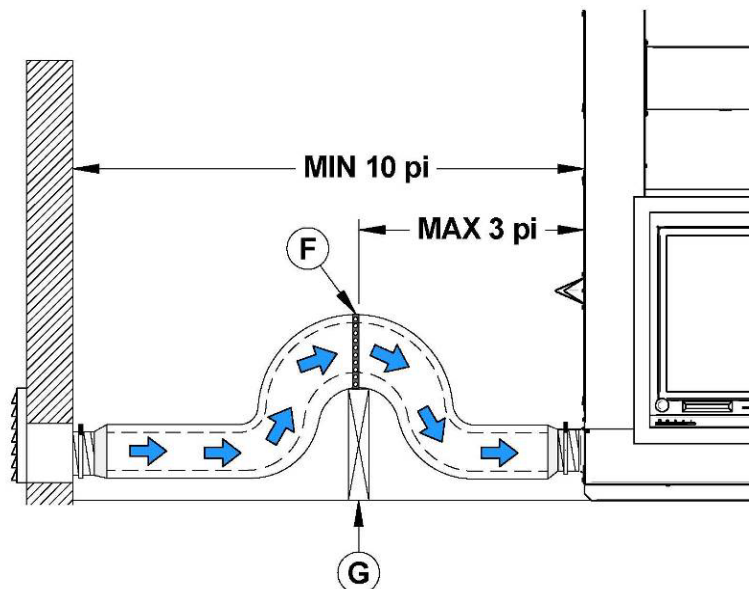
Figure 5 : P-Trap Example
