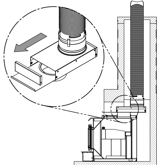
Figure 39: Offset liner adaptor
