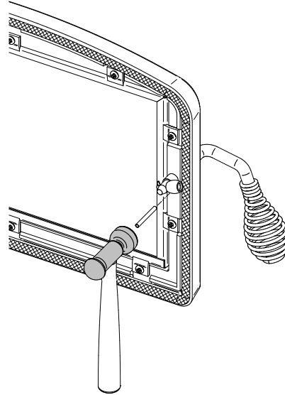
Figure 24: Installing the split pin
