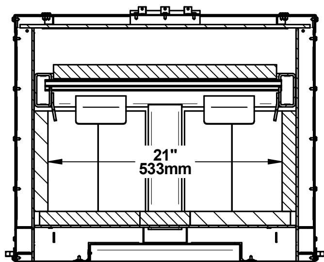
Figure 7: Front Firebox
