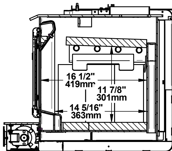
Figure 6: Side Firebox
