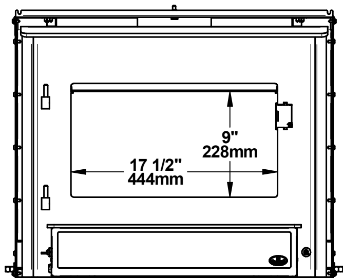
Figure 5: Door Opening
