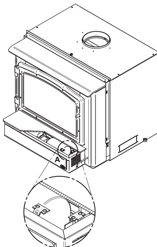
DETAIL A
