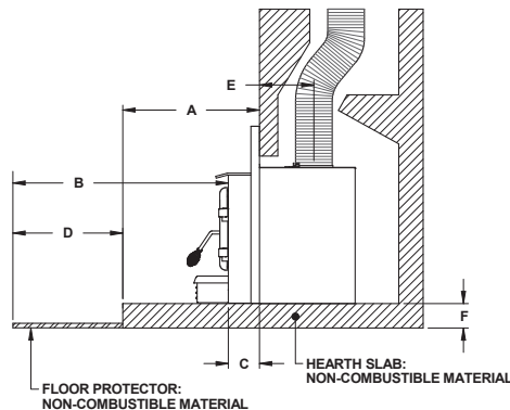
Figure 31: More than 5" raised base installation
