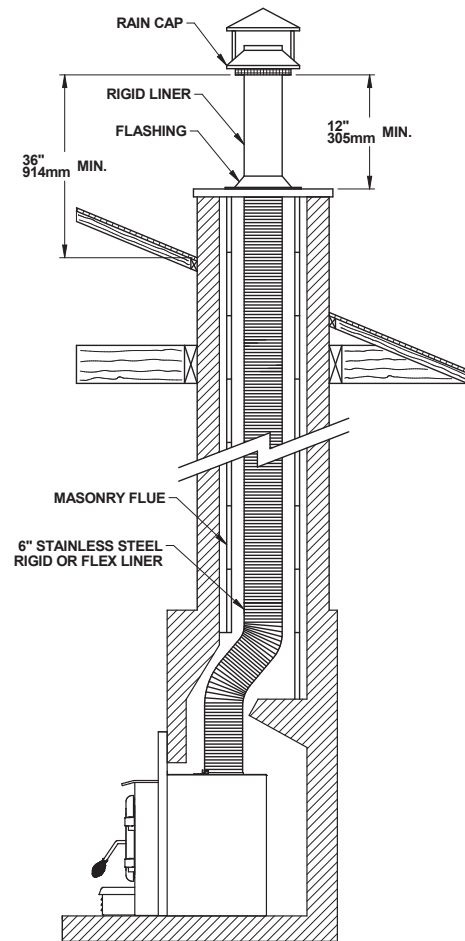
Figure 35: Liner Installation
