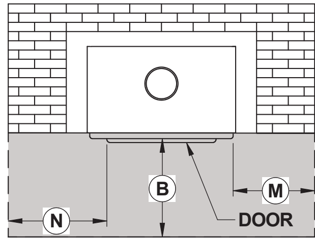
Figure 28: Floor Protection
