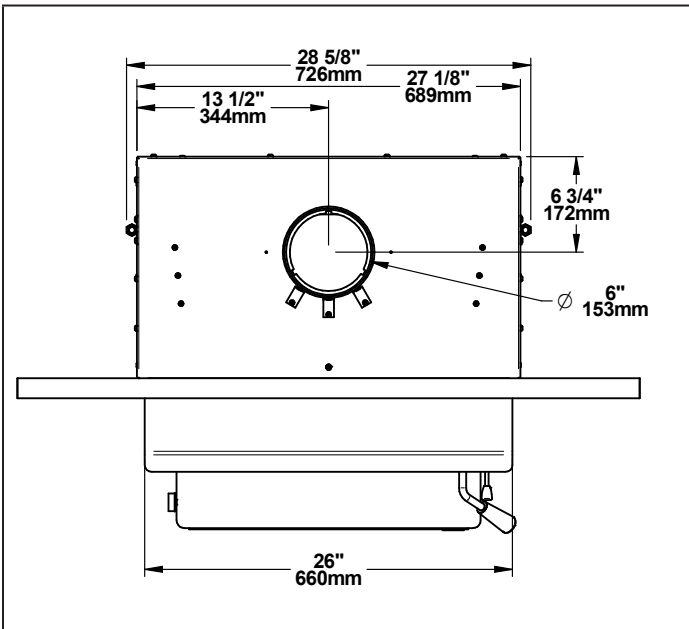
Figure 1: Top View
