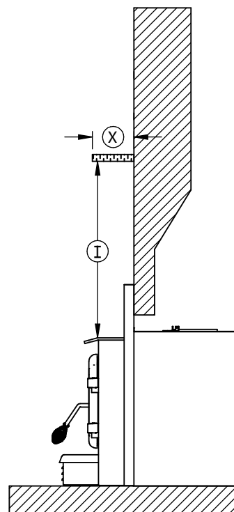
Figure 27: Shelf Clearances
