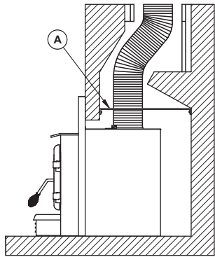
Figure 33: Block-off Plate
