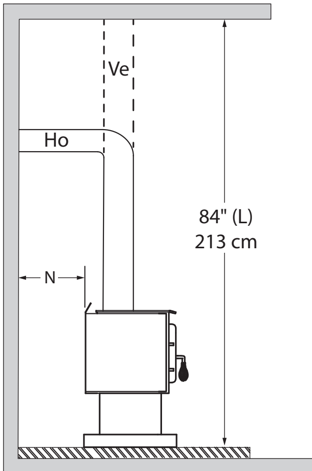
Figure 25: Clearances - Side
