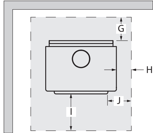
Figure 26: Floor Protection
