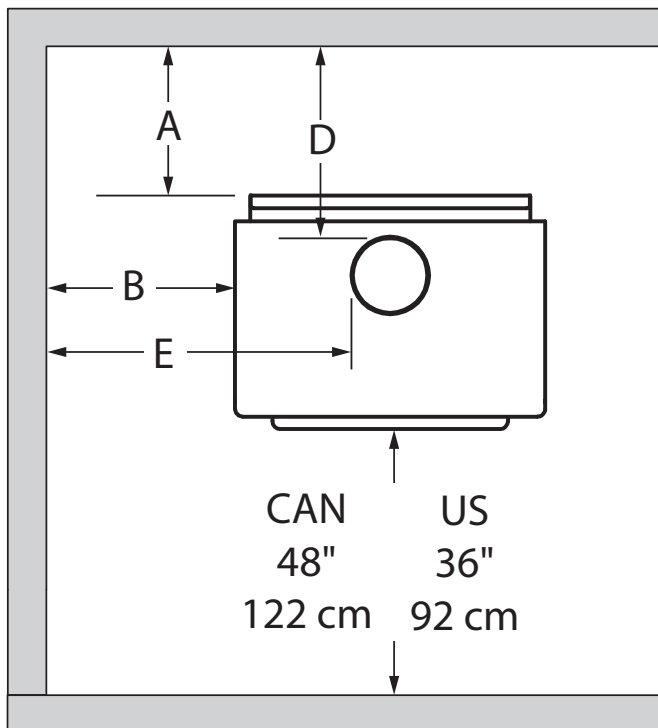
Figure 23: Clearances - Top
