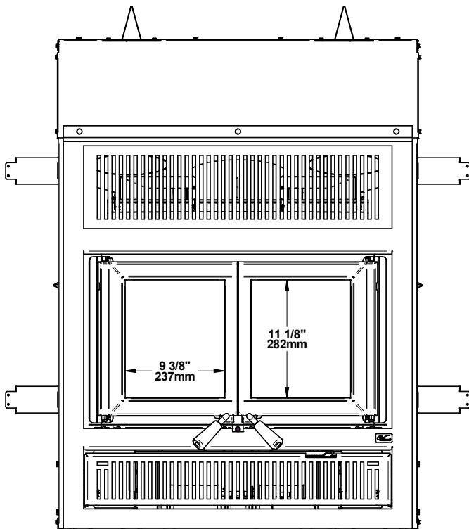
Figure 2: Front View
