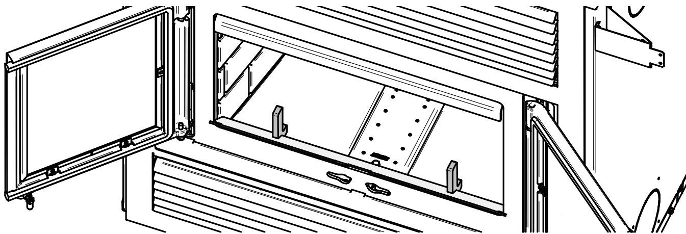
Figure 9: Reteneurs de bûches
