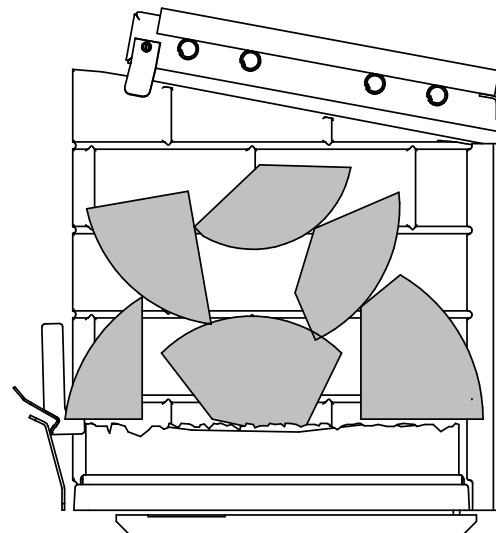
Figure 27: Low-burn rate load configuration - Side view
