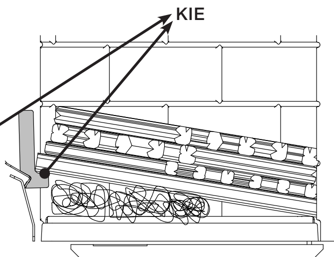
Figure 14: Kindling configuration using Kindling Ignition Enhancer (KIE) - Side view
