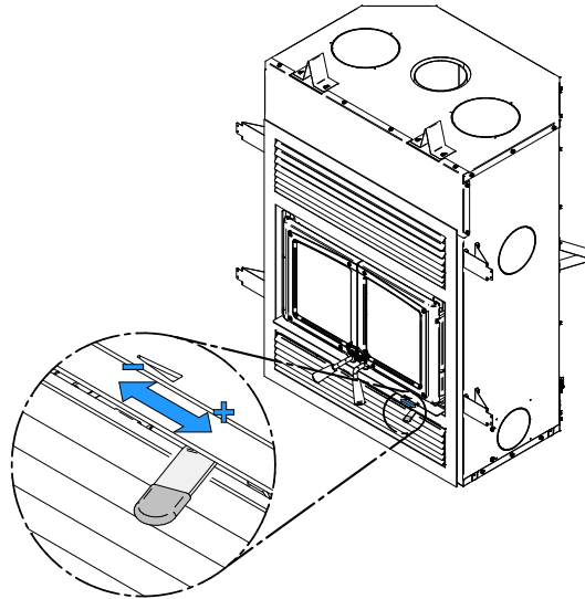
Figure 11: Air control
