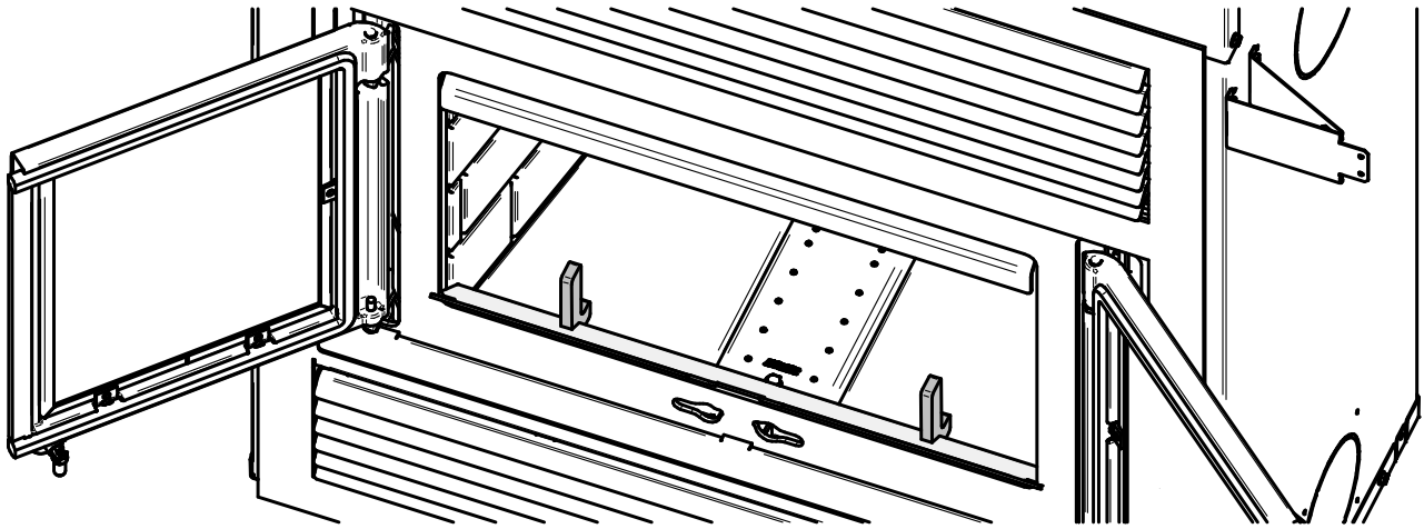
Figure 9: Log retainers
