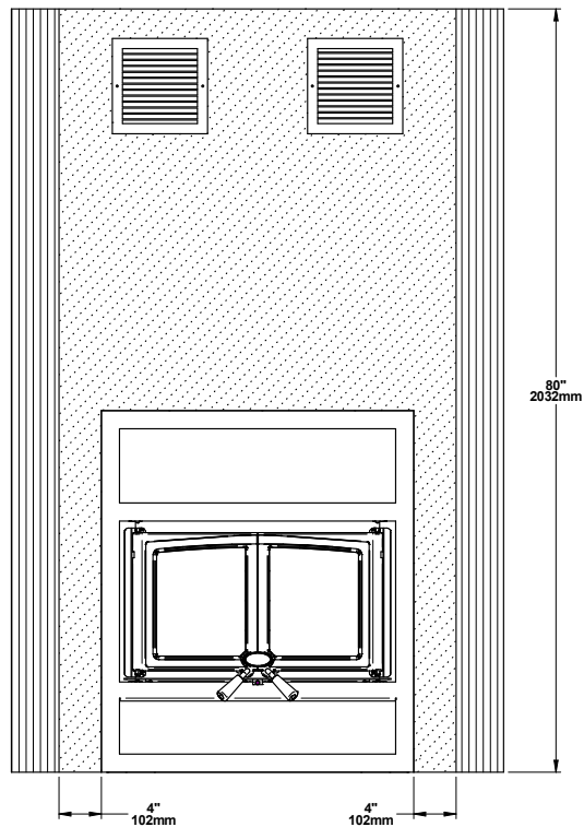
Unit with Hot air gravity kit
