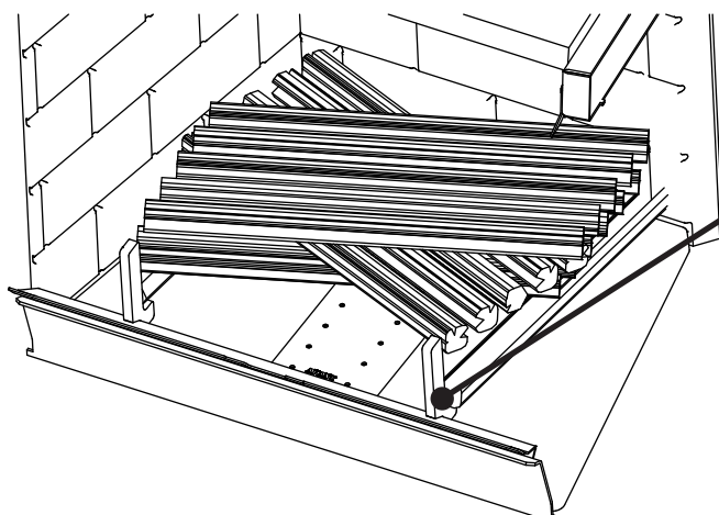
Figure 13: Kindling configuration using Kindling Ignition Enhancer (KIE) - Top view
