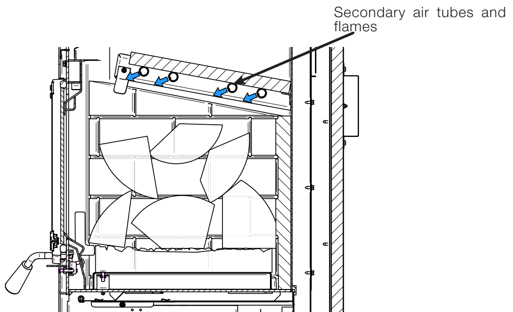
Figure 12: Secondary flame
