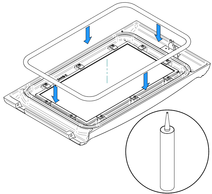
Figure 35: Gasket
