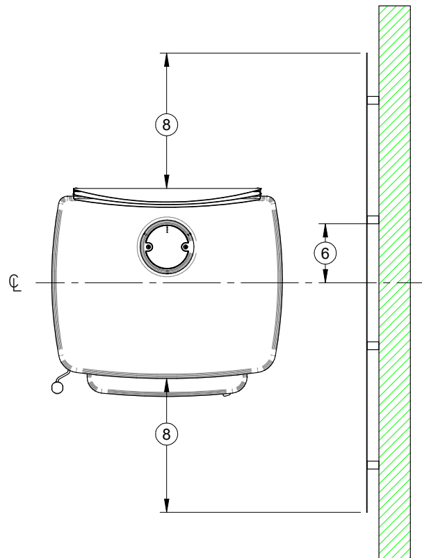
Figure 43: Clearances with Heat Shield - Top
