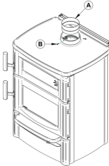
Figure 56: Universal connector PL36899
