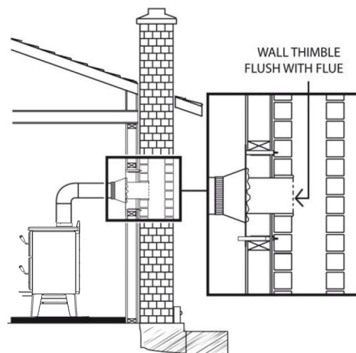
Figure 48: Masonry hearth installation
