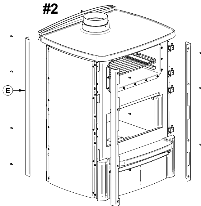
Figure 37: Remove the decorative panel moldings
