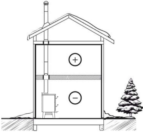
Figure 51: Good System Design
