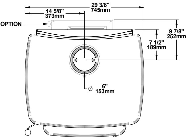
Figure 1: Top view
