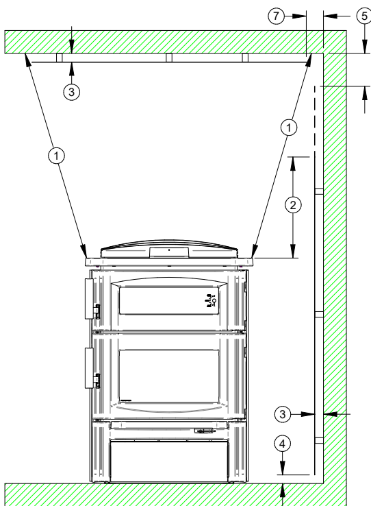
Figure 44: Clearances with Heat Shield - Face
