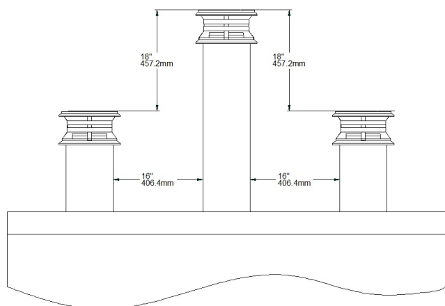
Figure 49: Flat roof
