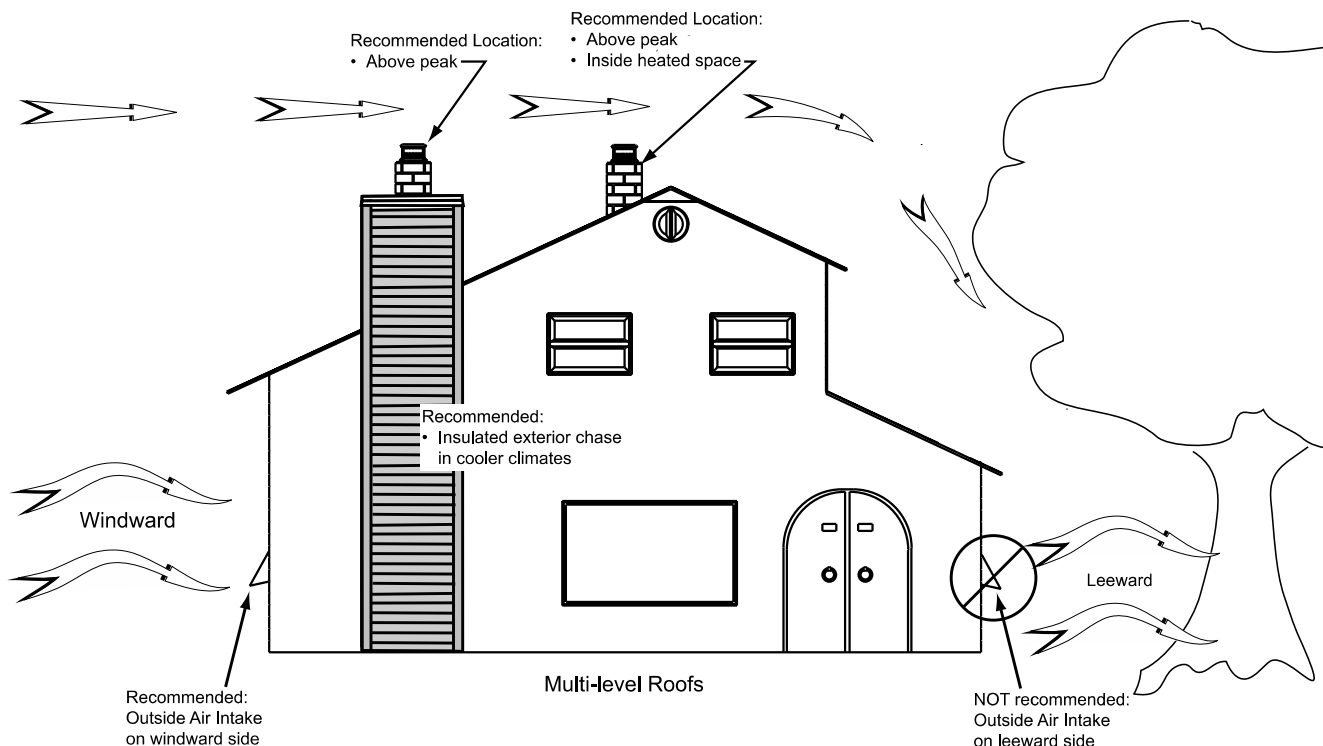
Figure 57: Air supply in conventional houses
