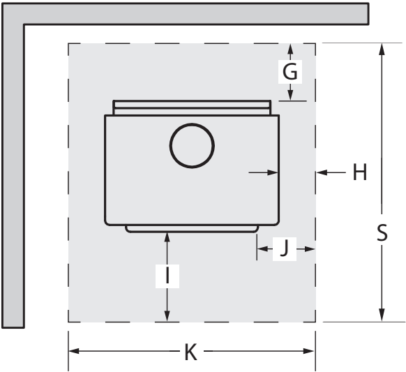
Figure 42: Floor protection
