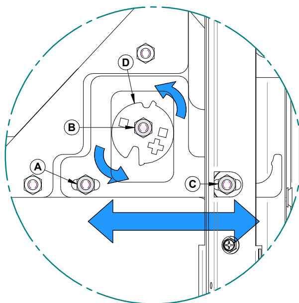
Figure 30: Oven door adjustment
