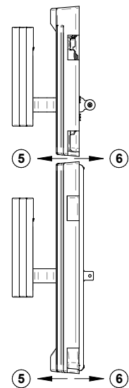
Figure 34: Eccentric hinges lateral adjustment
