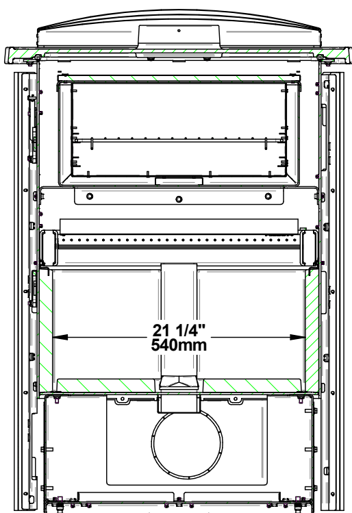
Figure 5: Front view : Combustion chamber
