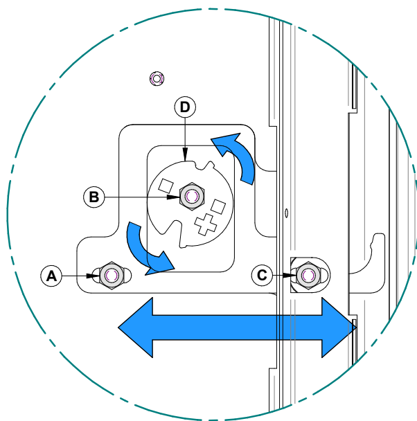
Figure 29: Combustion chamber door adjustment
