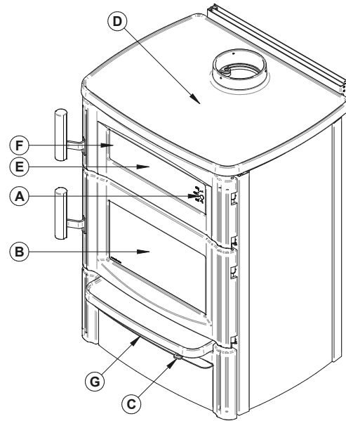
Figure 19: Component Location
