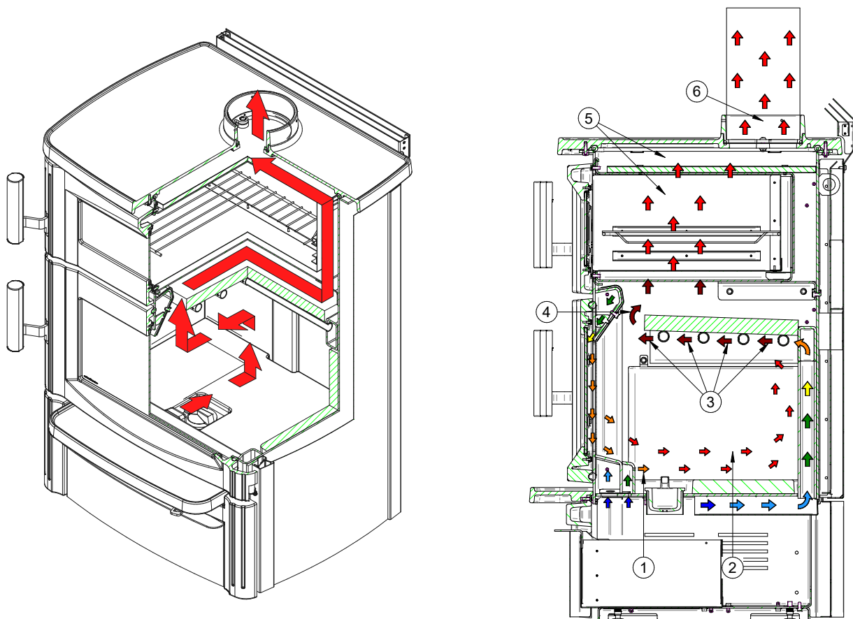
Figure 25: Gas path
