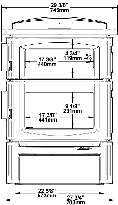
Figure 2: Front view
