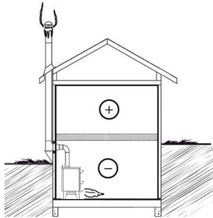
Figure 52: Acceptable System Design
