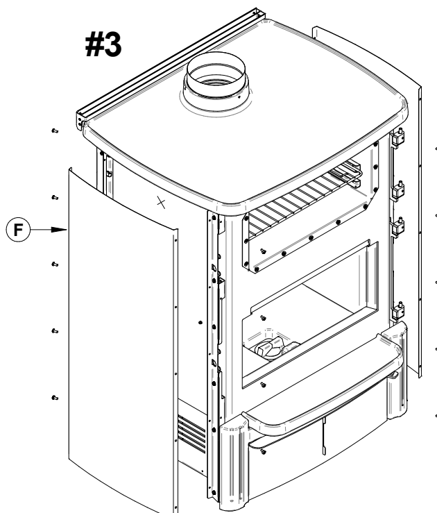
Figure 38: Remove the decorative panels
