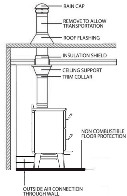
Figure 47: Mobile home installation
