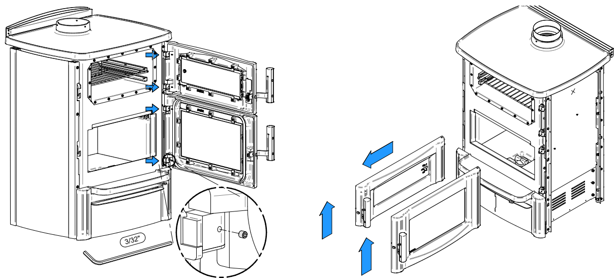
Figure 31: Release eccentric hinges
