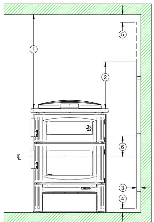
Figure 45: Clearances with Heat Shield - Face
