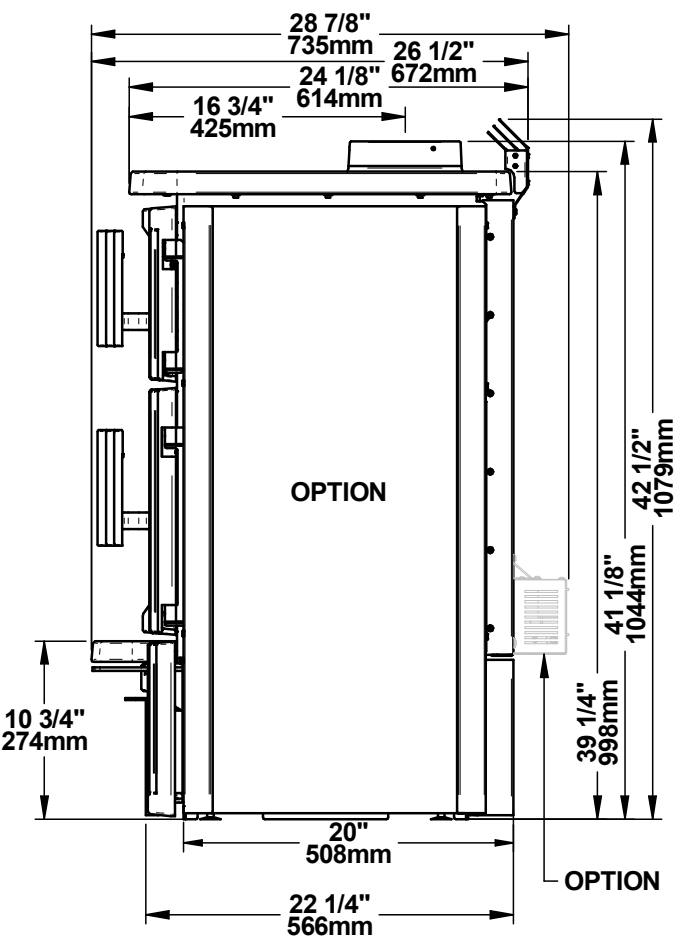
Figure 3: Side view
