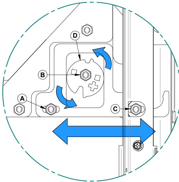
Figure 30: Ajustement porte de four
