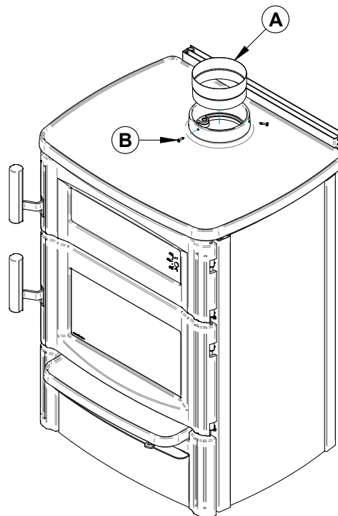
Figure 56: Raccord universel PL36899
