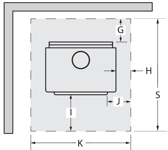
Figure 42: Protection de plancher
