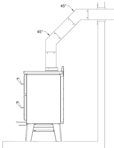
Figure 54: Acceptable
