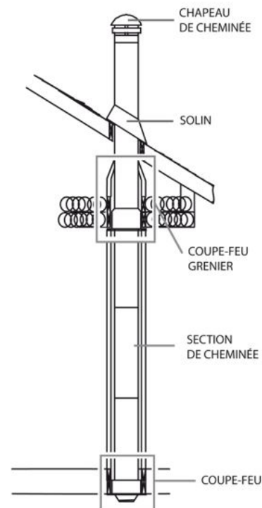
Figure 46: Installation standard
