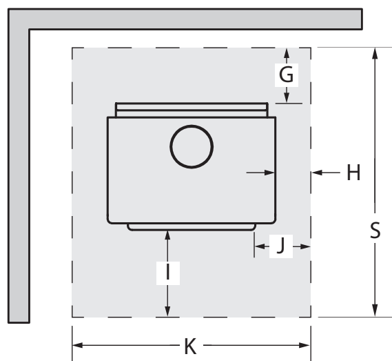
Figure 42: Protection de plancher
