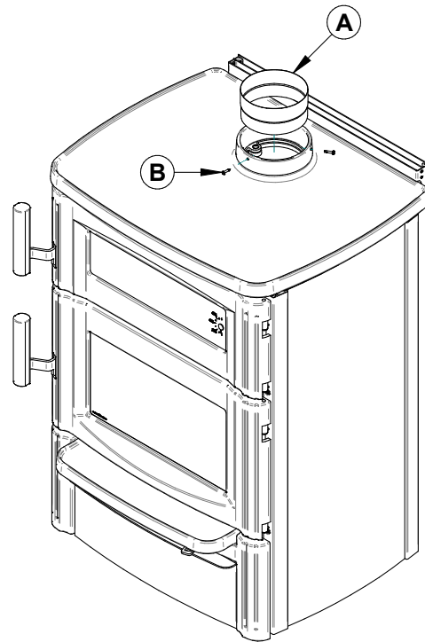
Figure 56: Raccord universel PL36899
