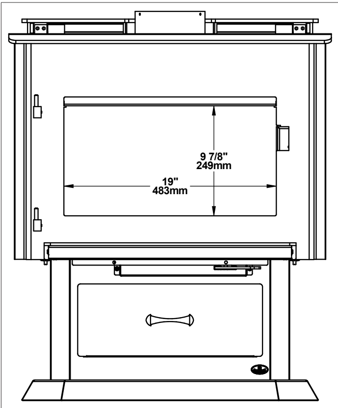
Figure 4: Door Opening
