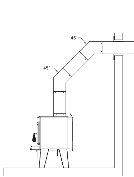
Figure 21: Acceptable
