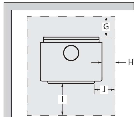
Figure 16: Floor Protection
