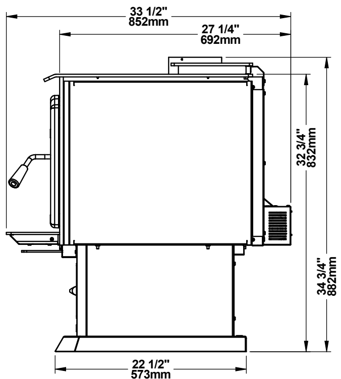
Figure 3: Side View
