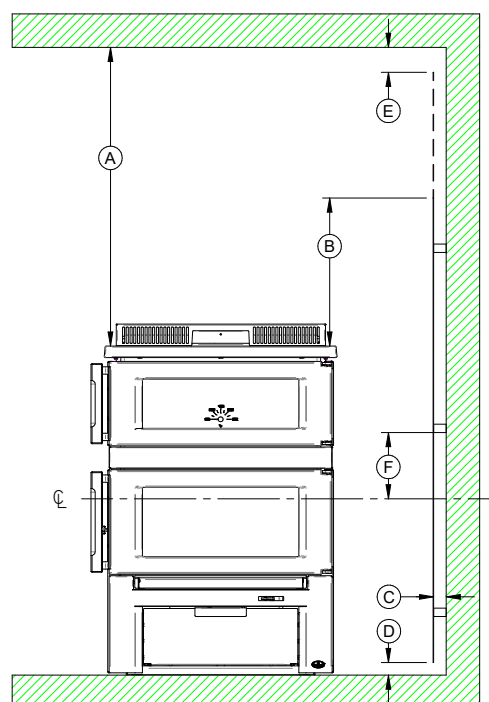
Figure 46: Clearances with Heat Shield - Face
