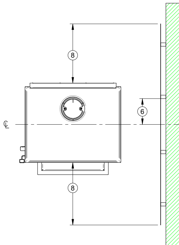
Figure 44: Clearances with Heat Shield - Top
