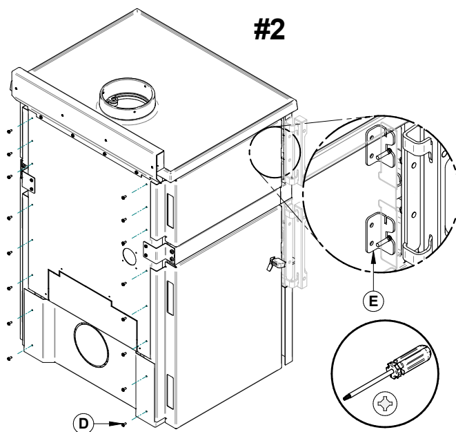
Figure 38: Decorative panels support
