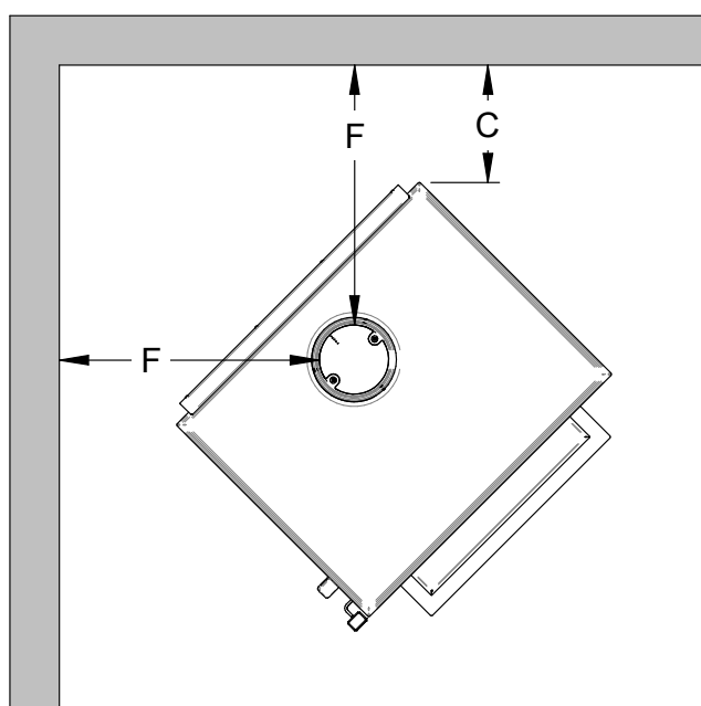
Figure 42: Clearances - Corner
