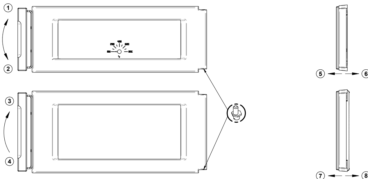
Figure 33: Eccentric hinges depth adjustment
