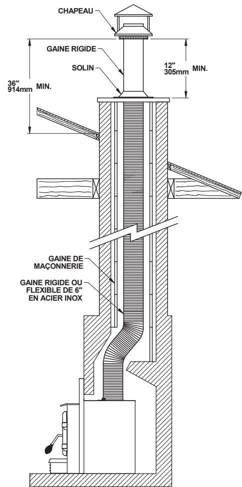
Figure 16: Installation de la gaine
