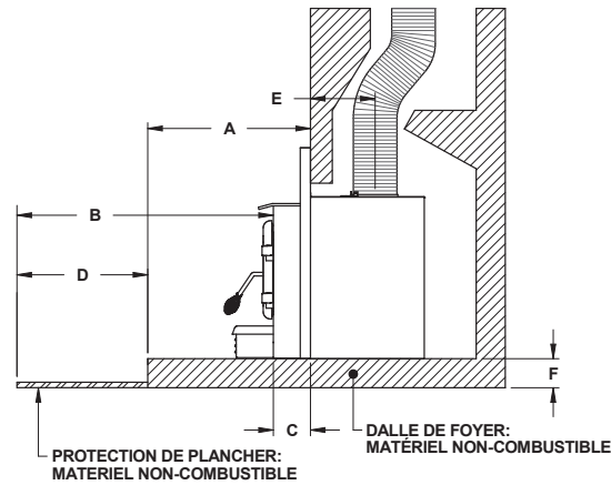
Figure 29: Protection de plancher additionnelle
