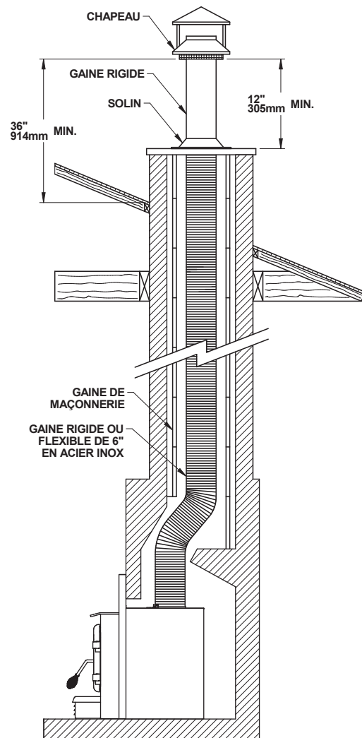
Figure 35: Installation de la gaine
