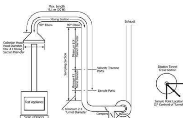
FIGURE 1 – DILUTION TUNNEL
