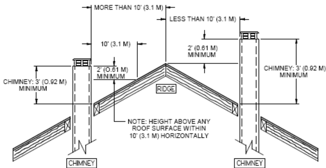
Figure 42 : Slope Roof
