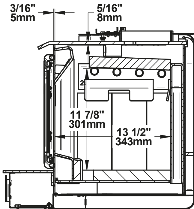
Figure 7 : Side View - Combustion Chamber
