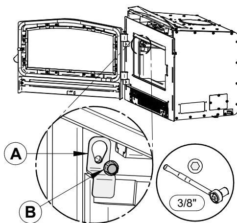
Figure 14 : Remove stone supports
