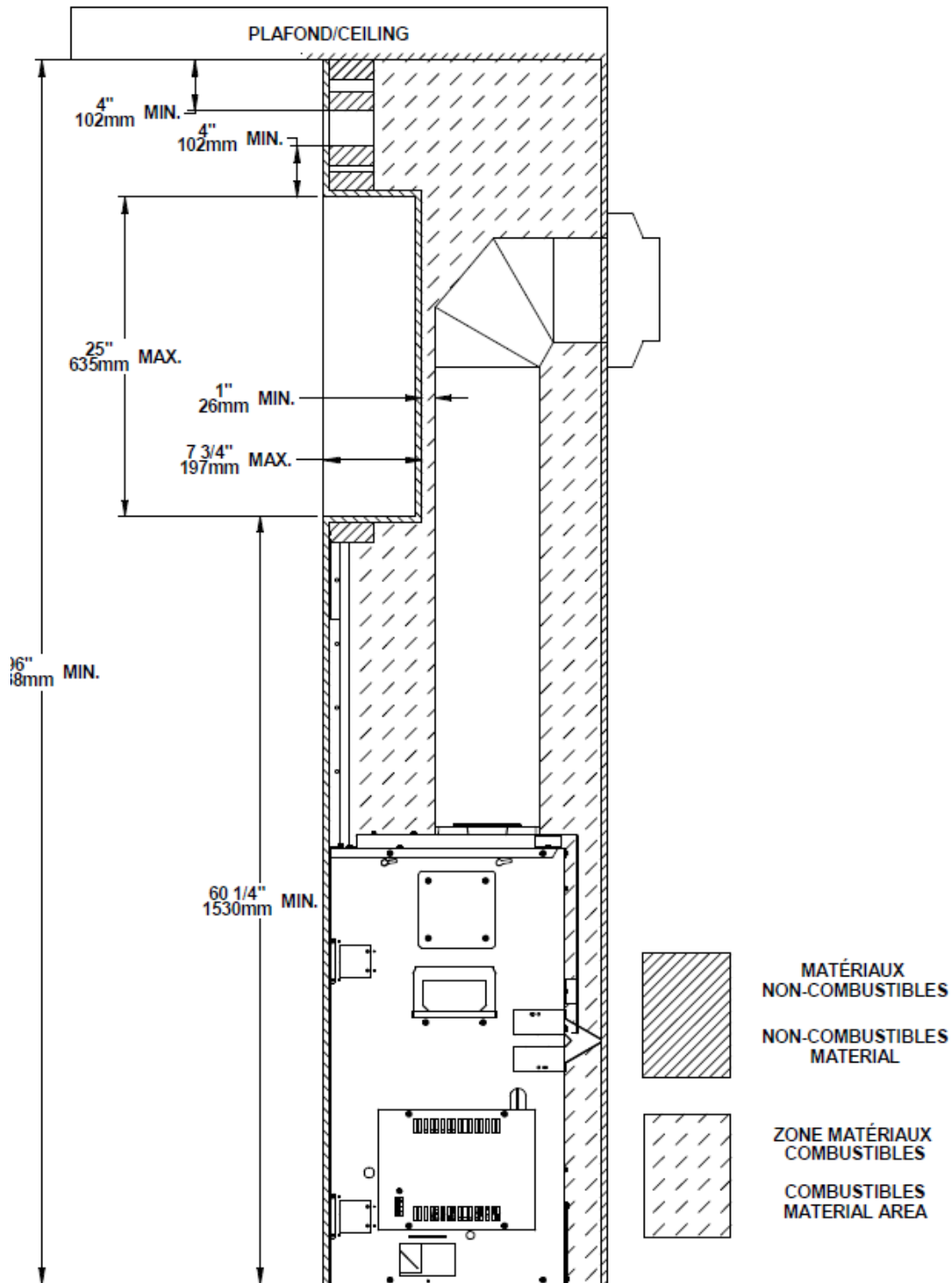
Figure 9 : Hot air vent kit positioning with television recess
