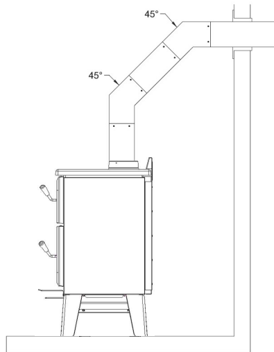
Figure 38: Acceptable
