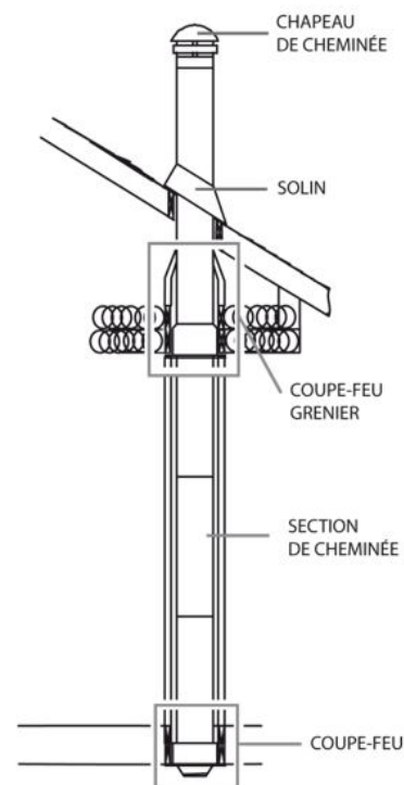
Figure 30: Installation standard
