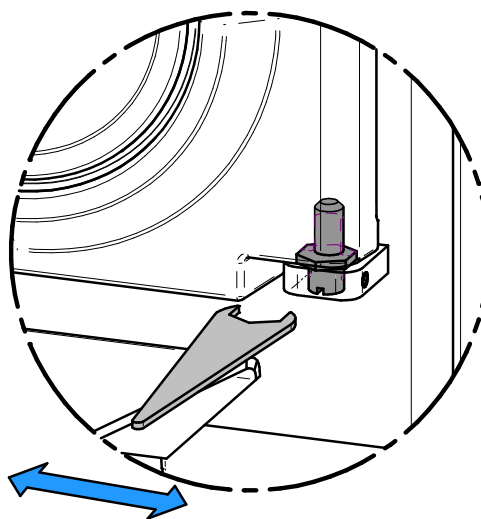
Figure 16: Ajuster les pentures excentriques
