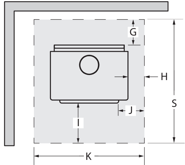
Figure 24: Protection de plancher
