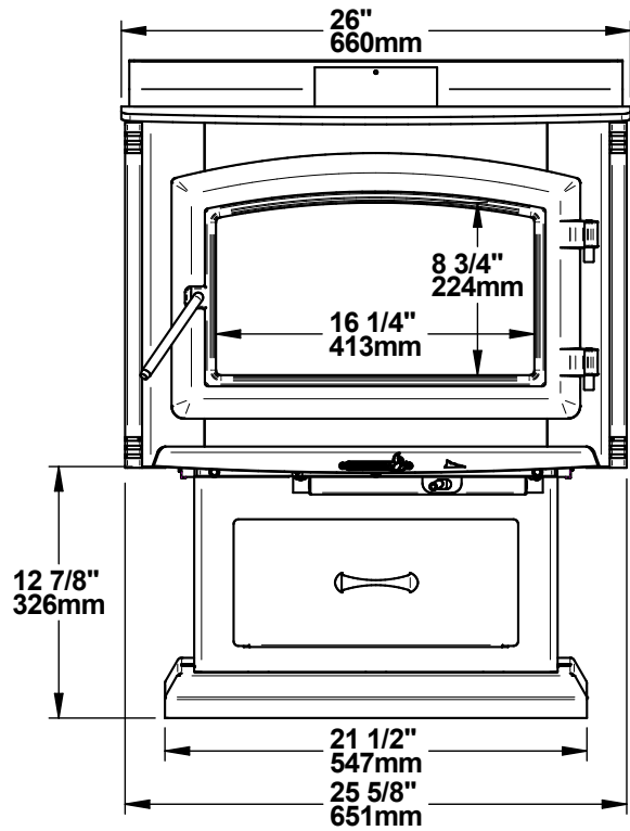
Figure 11: Front view
