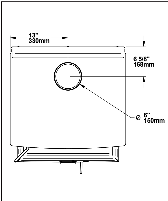
Figure 10: Top view
