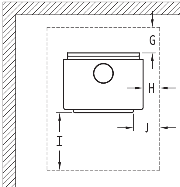
Figure 26: Floor Protection
