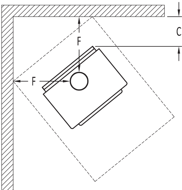
Figure 25: Clearances - Corner
