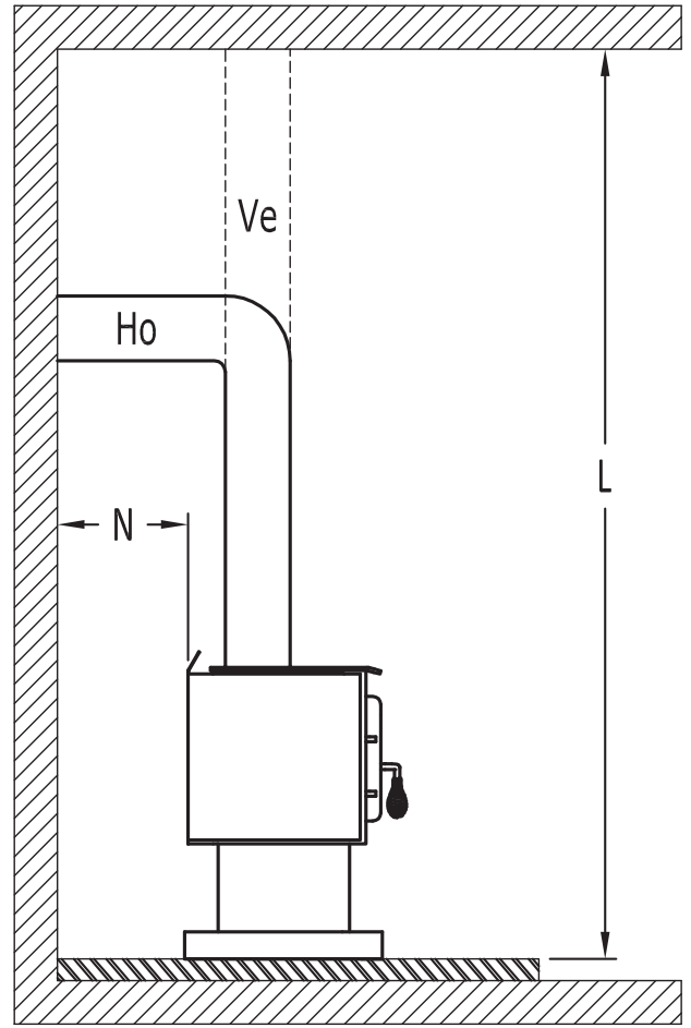
Figure 24: Clearances - Top
