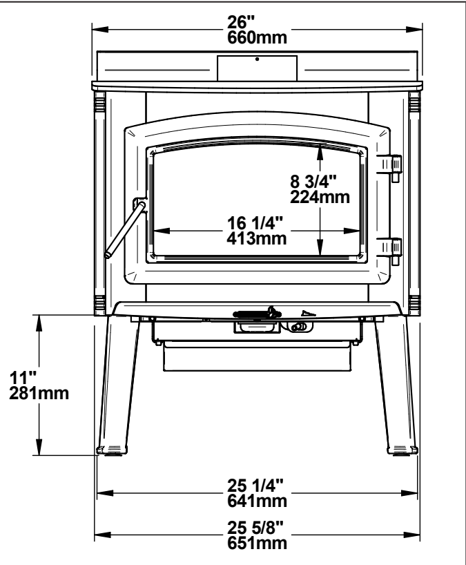
Figure 8: Front view
