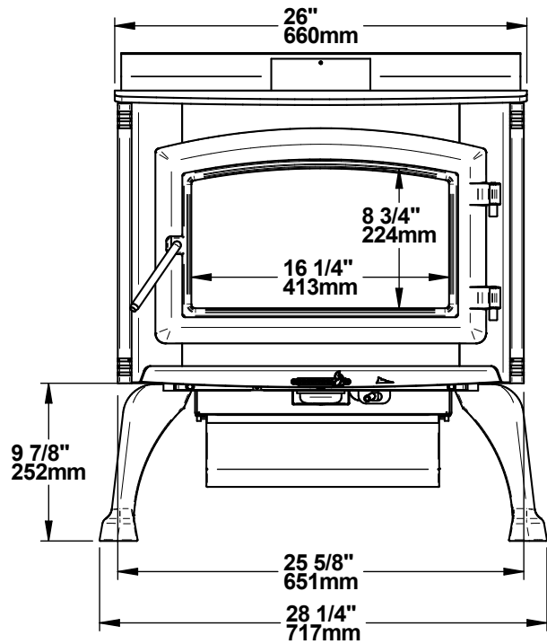
Figure 2: Front view
