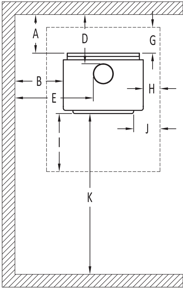
Figure 23: Clearances -Side
