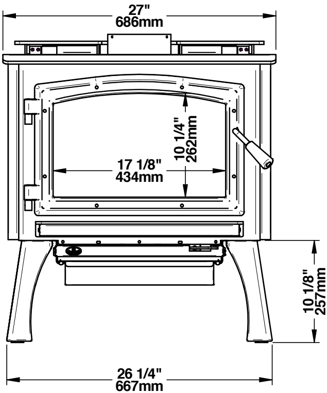
Figure 5: Front view
