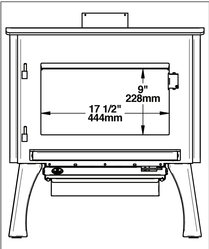
Figure 10: Door opening
