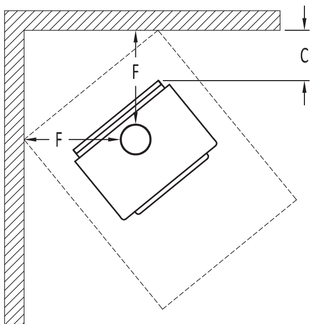
Figure 35: Clearances - Corner
