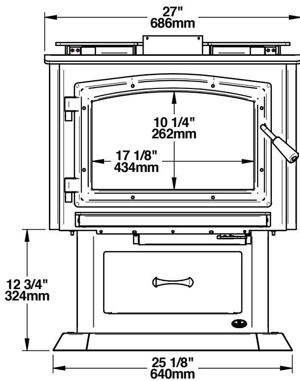
Figure 8: Front view
