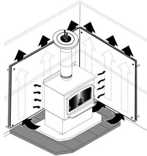
Figure 38: Heat shield
