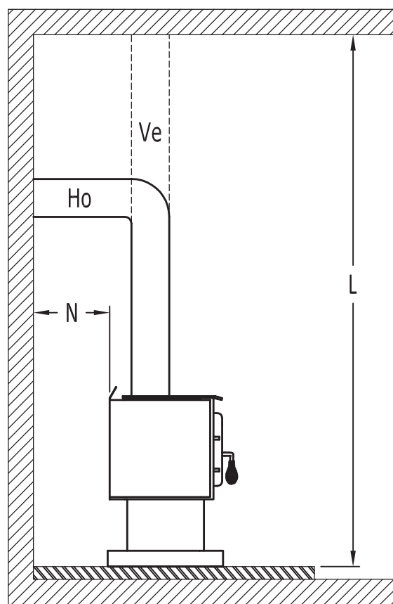
Figure 34: Clearances - Side
