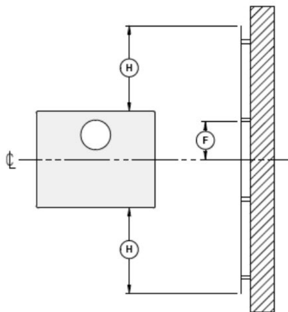
Figure 40: Heat shield clearances
