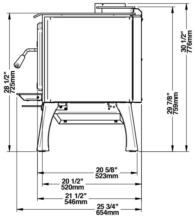
Figure 6: Side view
