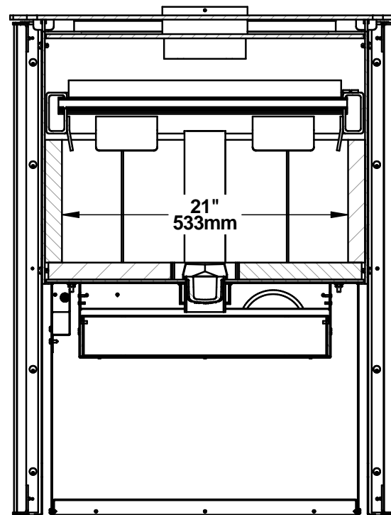
SECTION B-B
